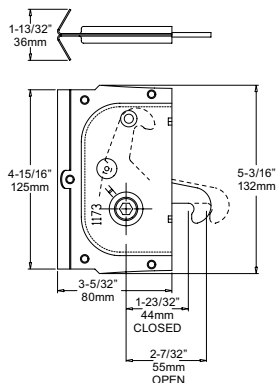
ITEM # 1173 LOCKING POINT
