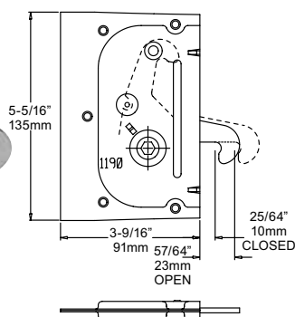
ITEM # 1190 LOCKING POINT
