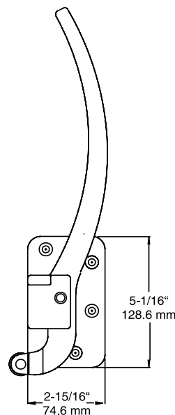
OUTSIDE RELEASE HANDLE
